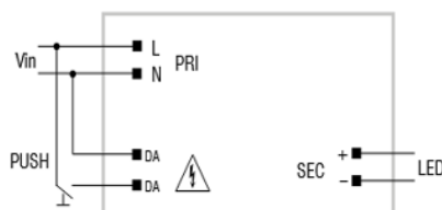
PUSH SWITCH diagram - Collegamento PUSH SWITCH
