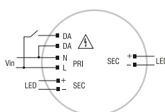
PUSH SWITCH diagram Collegamento PUSH SWITCH
