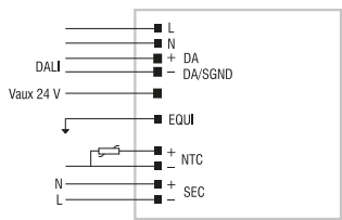
D4i wiring diagram Collegamento D4i
